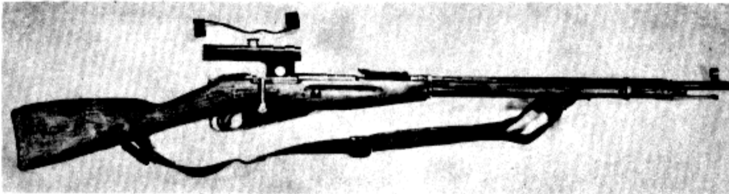
FIGURE 27. SNIPER RIFLE WITH PU TELESCOPE AND MOUNT (RIGHT SIDE).
